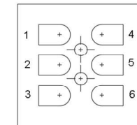
Socket view of screw terminals
